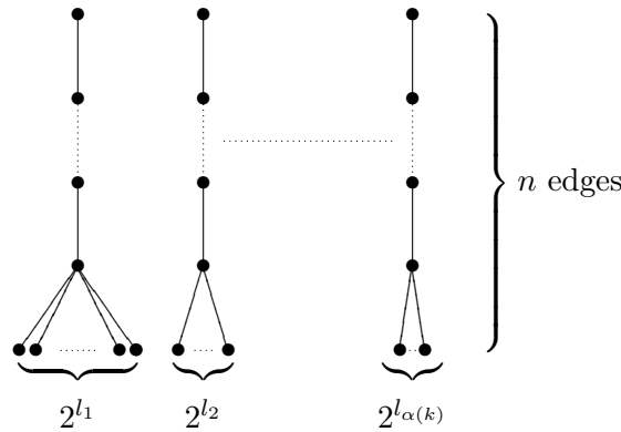
Figure 1: A collection of trees representing an additive generator in H^{(n-1)(k-\alpha(k))}(B(\mathbb{R}^n, k)) .
